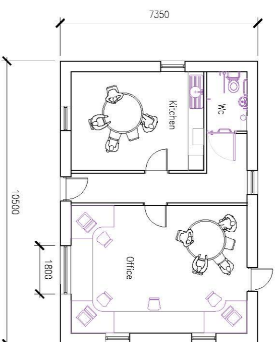
Low Level Plan Scale 1:100
