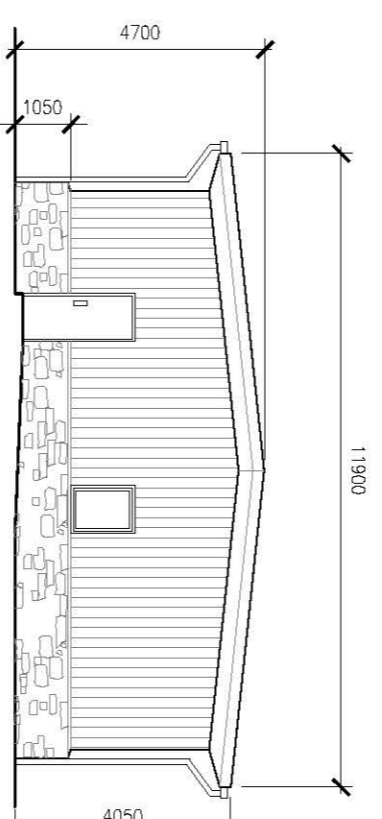
West Elevation Scale 1:100
