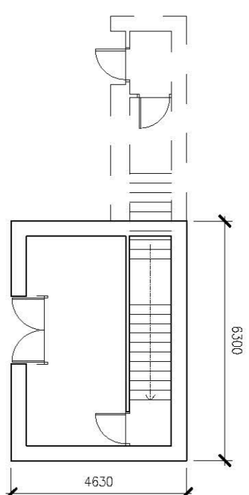
Sectional Plan Scale 1:100
