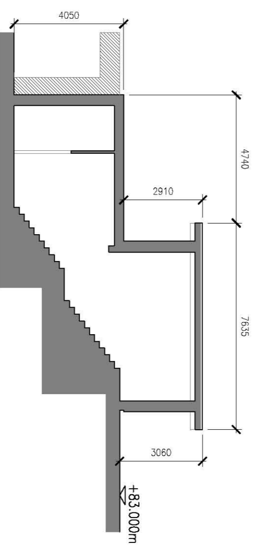
Section Scale 1:100
