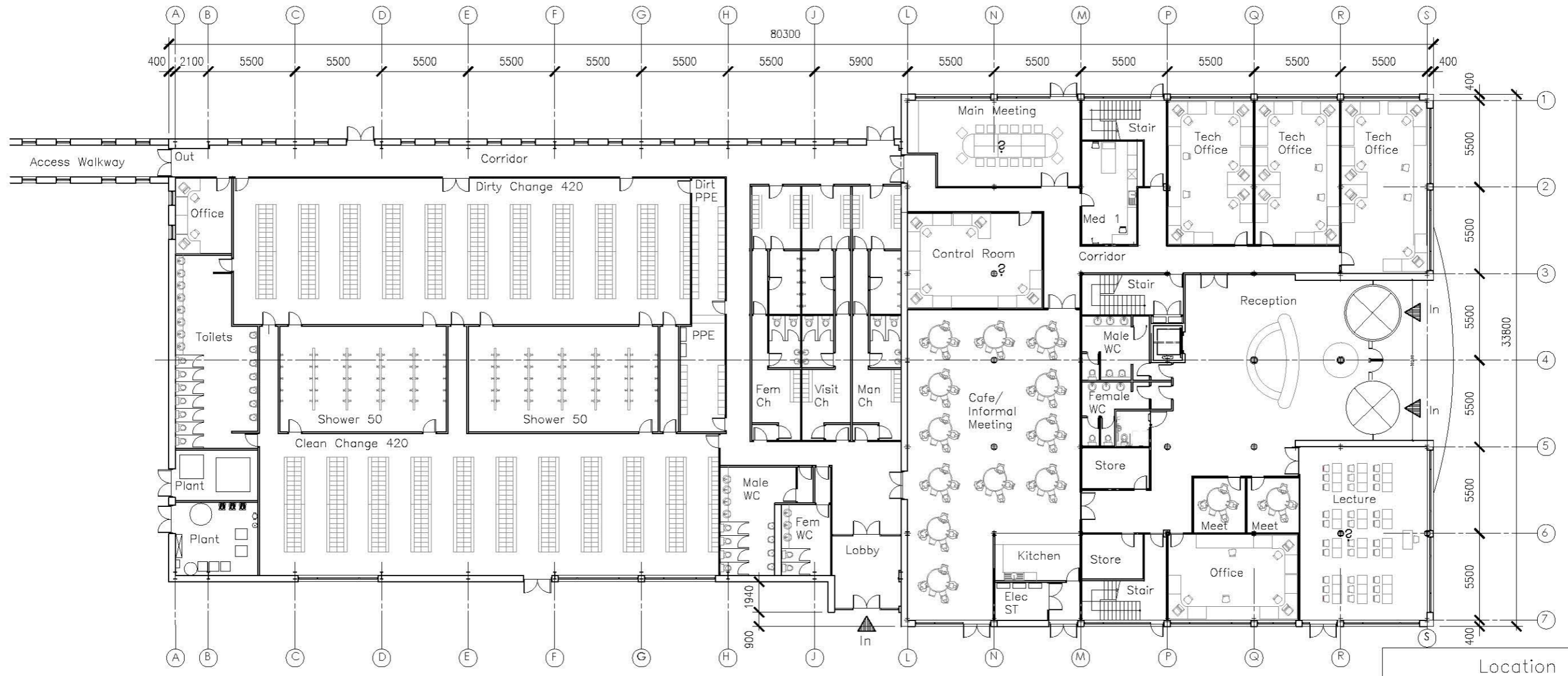
Ground Floor Scale 1:200
