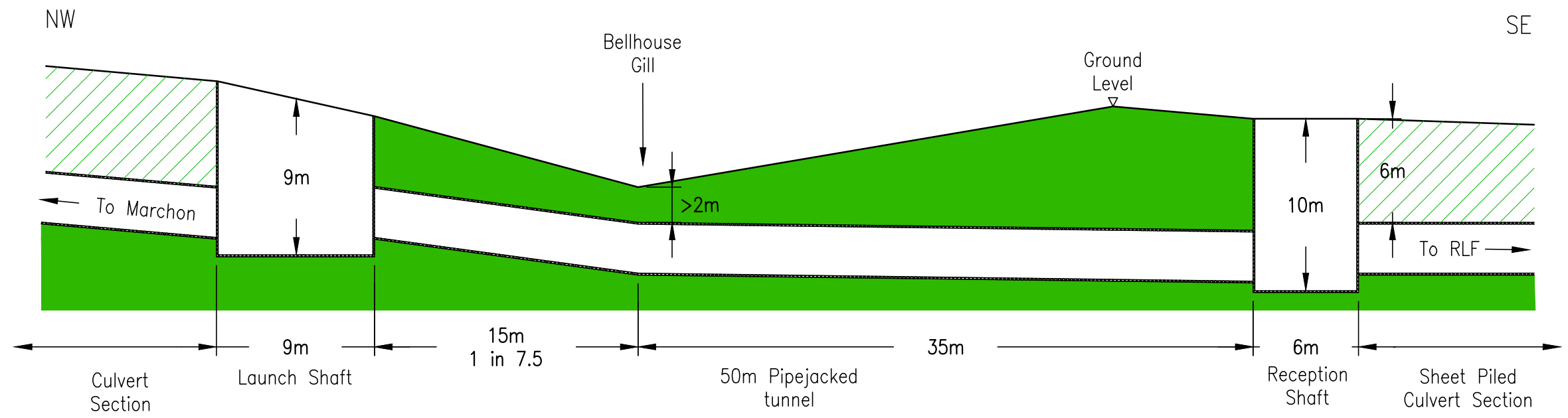
Bellhouse Gill Pipejacking Cross Section
