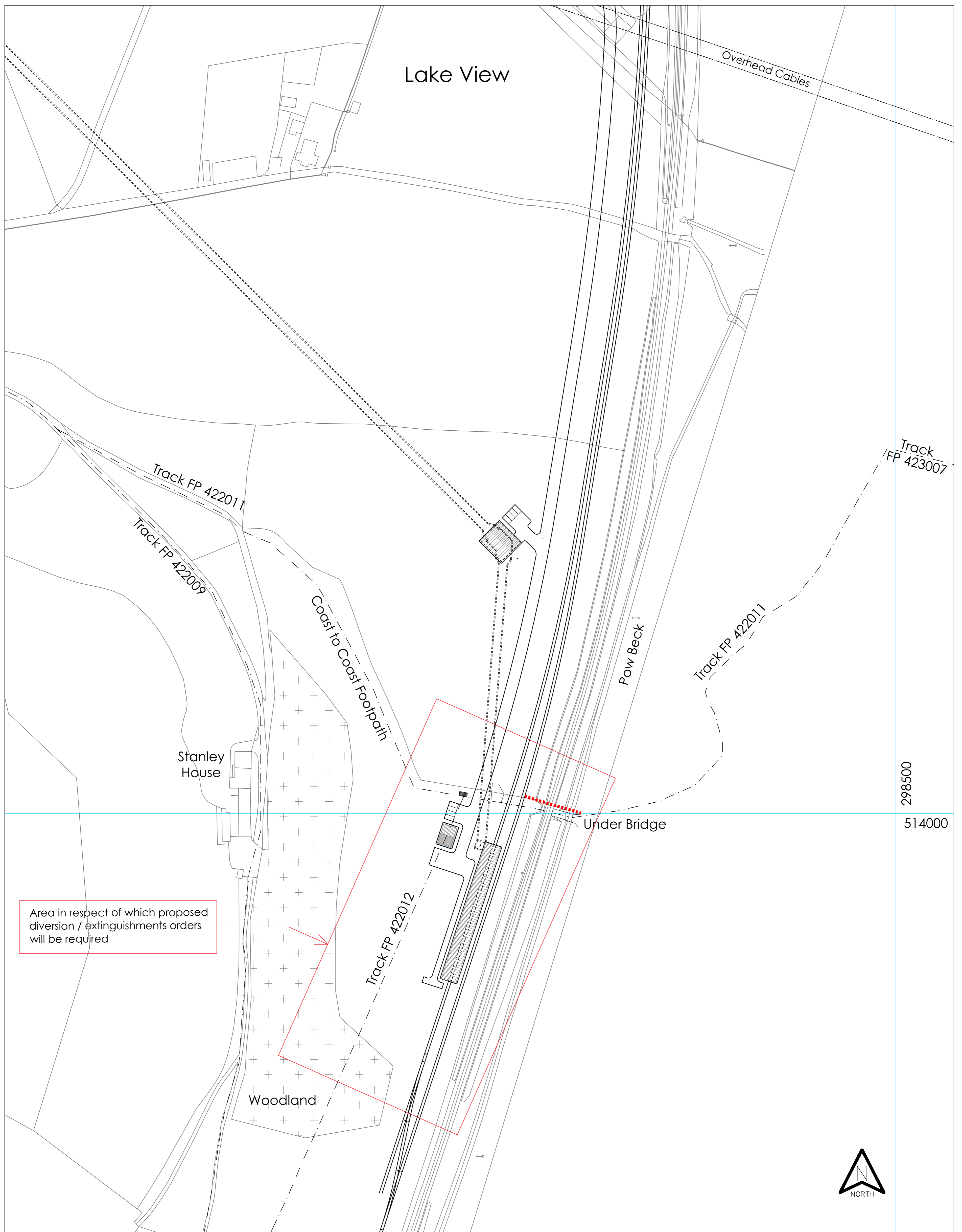
Plan of Eastern Outfall Drain Scale 1:1000
