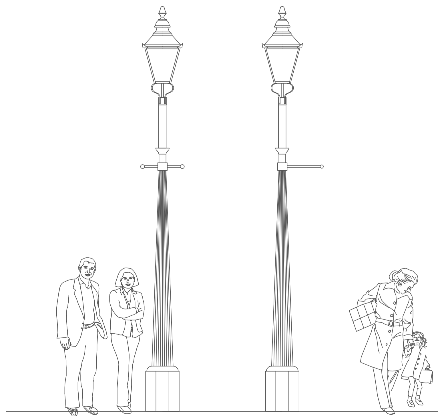
SCALE 1:25 - PROPOSED LIGHTING COLUMNS
